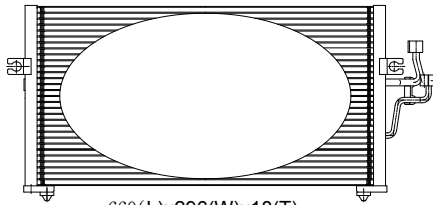
660(L)x296(W)x18(T)
