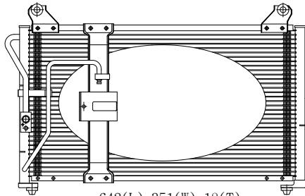
642(L)x351(W)x18(T)
