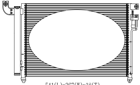
541(L)x367(W)x18(T)
