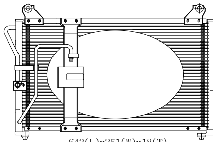
642(L)x351(W)x18(T)
