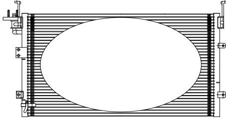
720(L)x349(W)x18(T)
